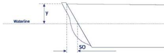
TRADITIONAL TRANSOM HUNG RUDDER
