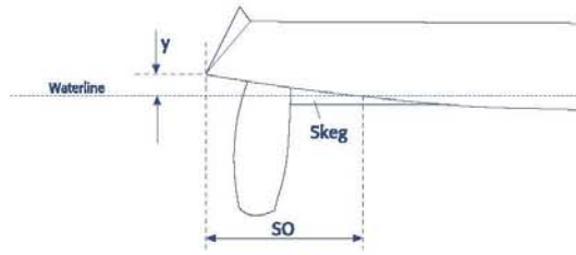
SPADE RUDDER
